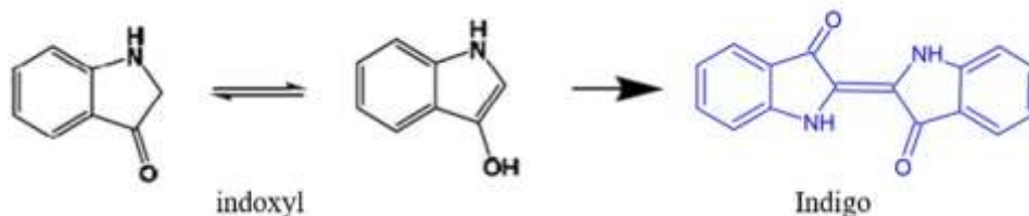
Figure 2. Structural transformation of indoxyl into indigo
