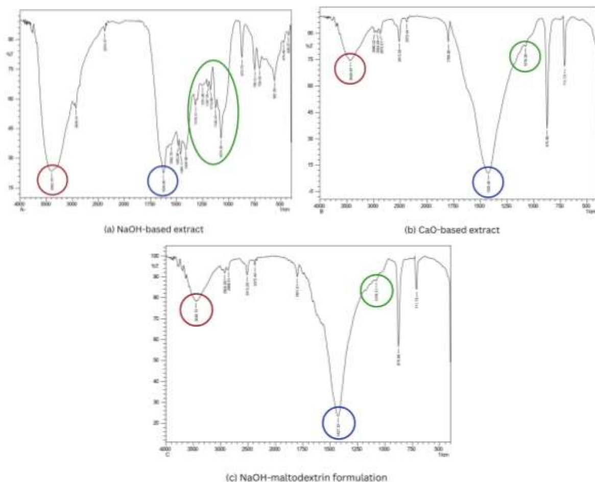
Figure 7. Comparative FTIR spectra of Strobilanthes cusia leaf extracts: (a) NaOH-based extract (b) conventional CaO-based extract, and (c) the formulated NaOH-maltodextrin paste.
