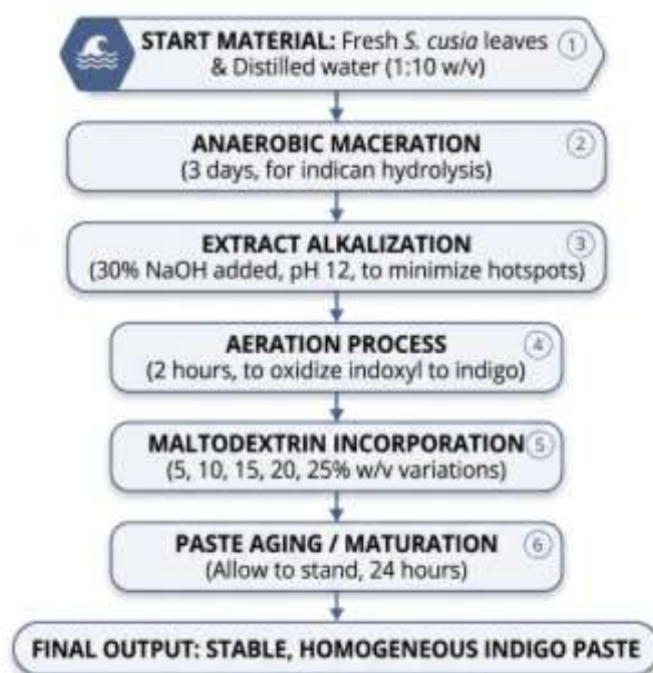
Figure 3. Systematic flowchart of the maceration, alkalization, and aeration process for Strobilanthes cusia indigo paste formulation
