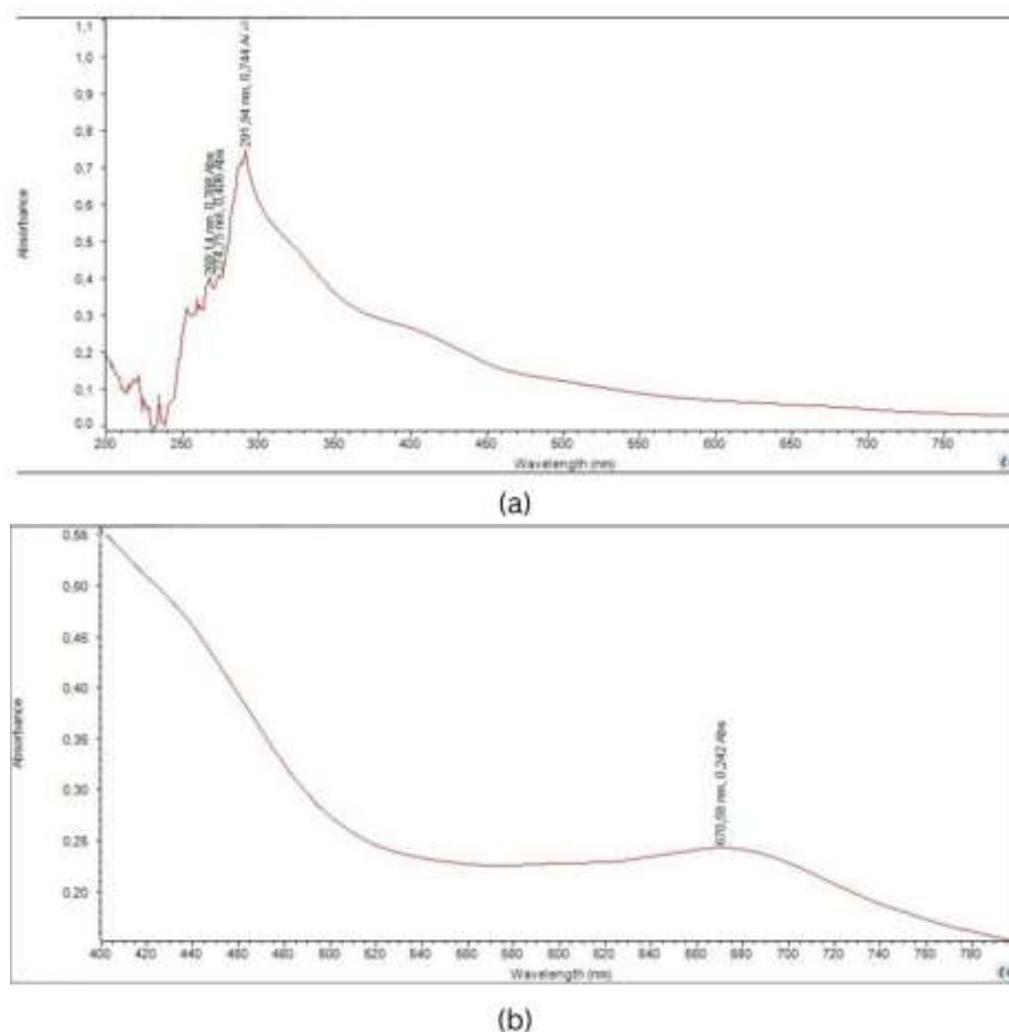
Figure 6. UV-Visible absorption spectra tracking the pigment transformation: (a) fresh Strobilanthes cusia leaf maceration liquor indicating precursors at 291.94 nm, and (b) the aerated extract confirming indigo chromophore formation at 670.58 nm.
