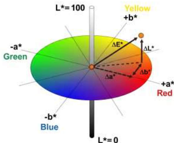
Figure 8. Illustration of the CIE L^*a^*b^* color space
