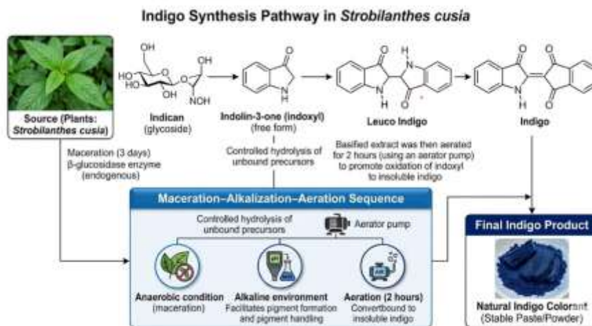
Figure 4. Integrated pathway of indigo synthesis and the sequential extraction process from Strobilanthes cusia
